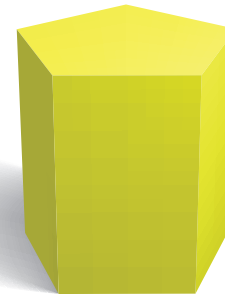
Pentagonal Prism
