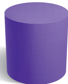
Cylinder
