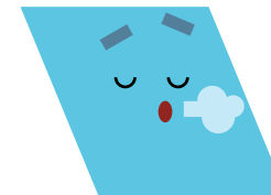
Parallelogram
