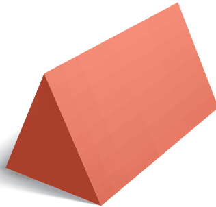
Triangular Prism
